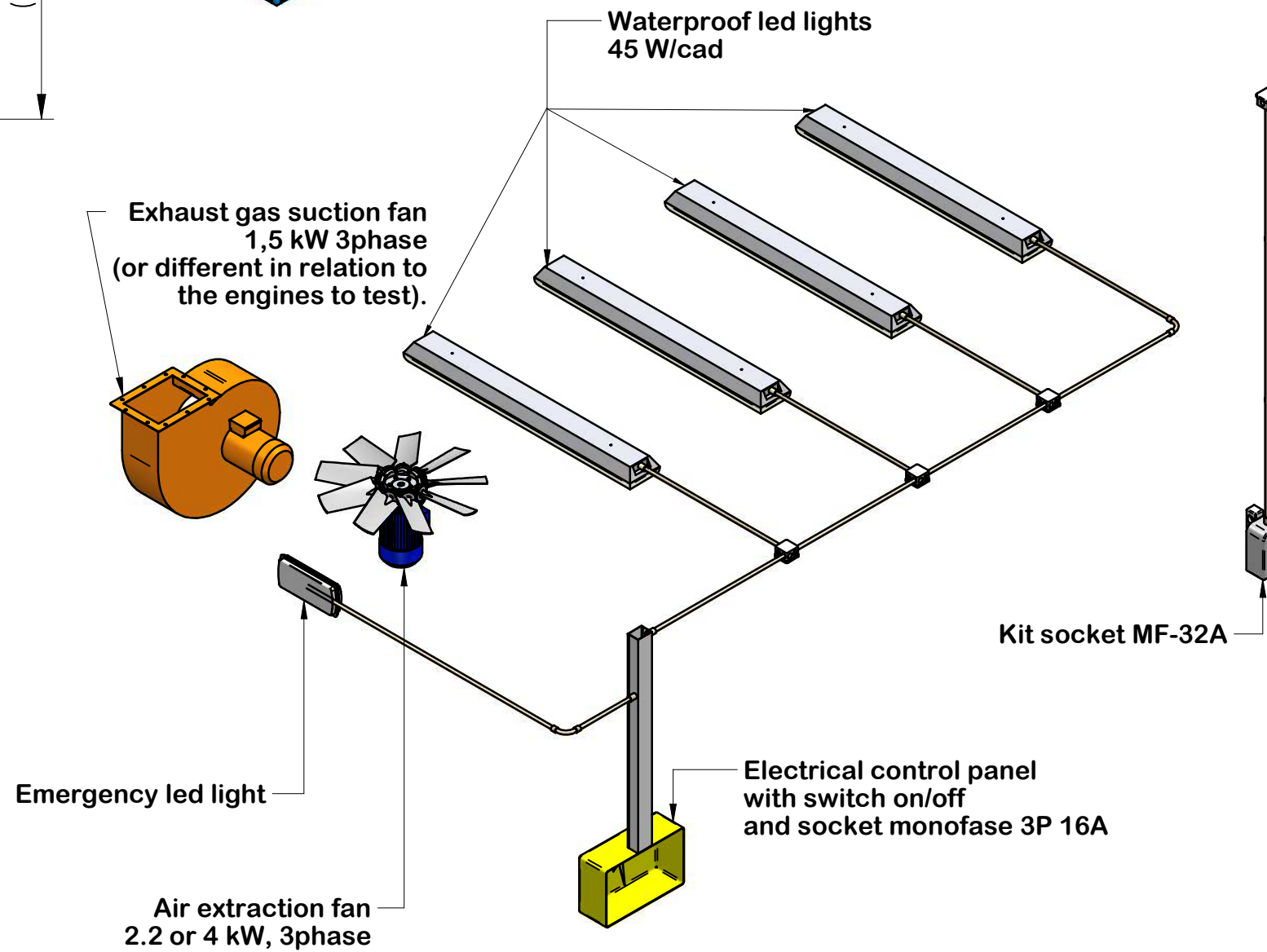
RIGHT SIDE
